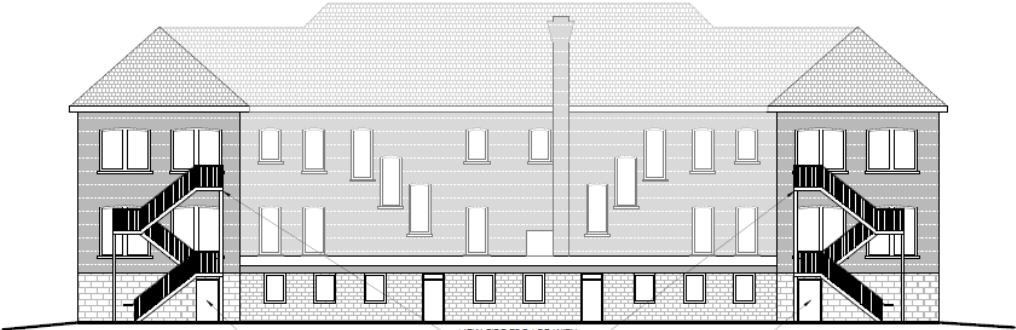
NORTH ELEVATION 1 2 5m
