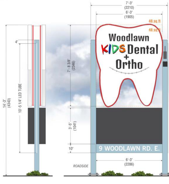
D/S Illuminated Pylon Sign Scale: 3/8"=1'-0"
