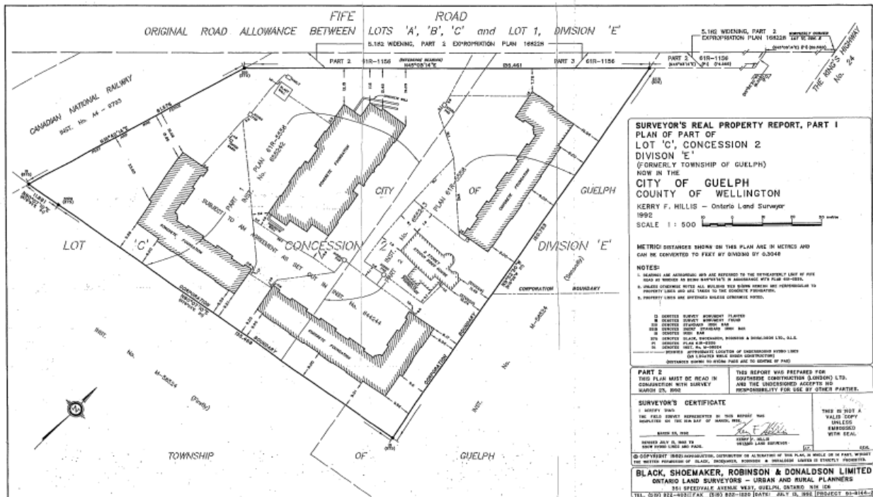
Figure 2 - Black and white surveyor's plan of subject property
