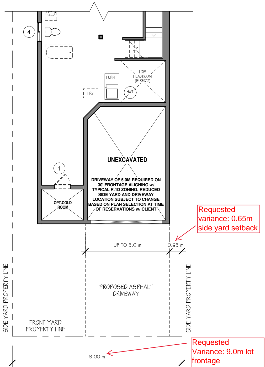
SITE PLAN
