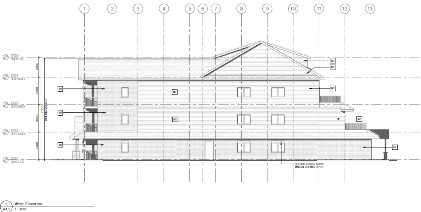
Figure 6: West Elevation
