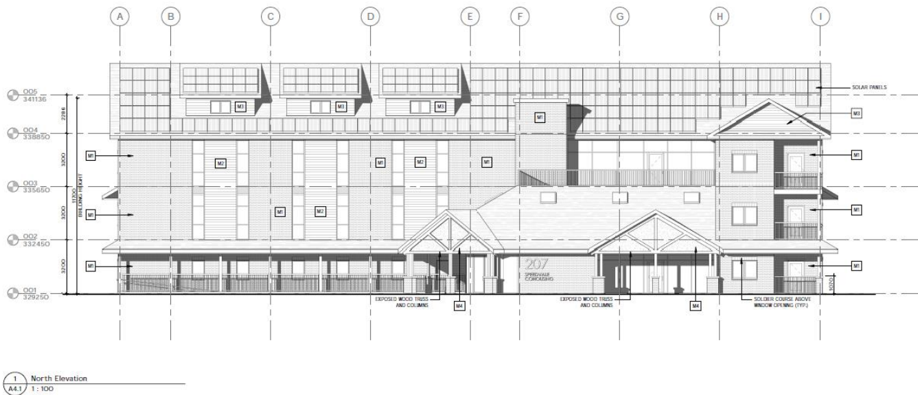
Figure 2: Front Elevation
