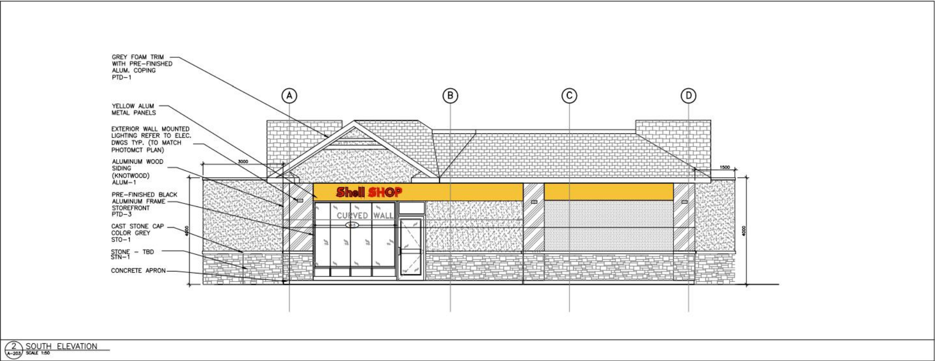
Figure 2: South Elevation
