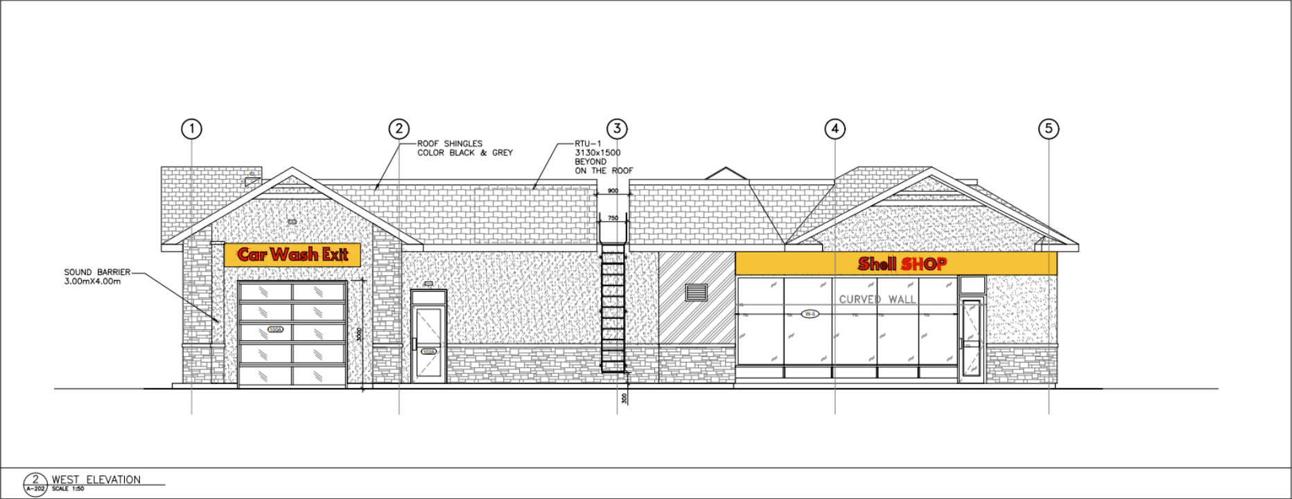
Figure 4: West Elevation
