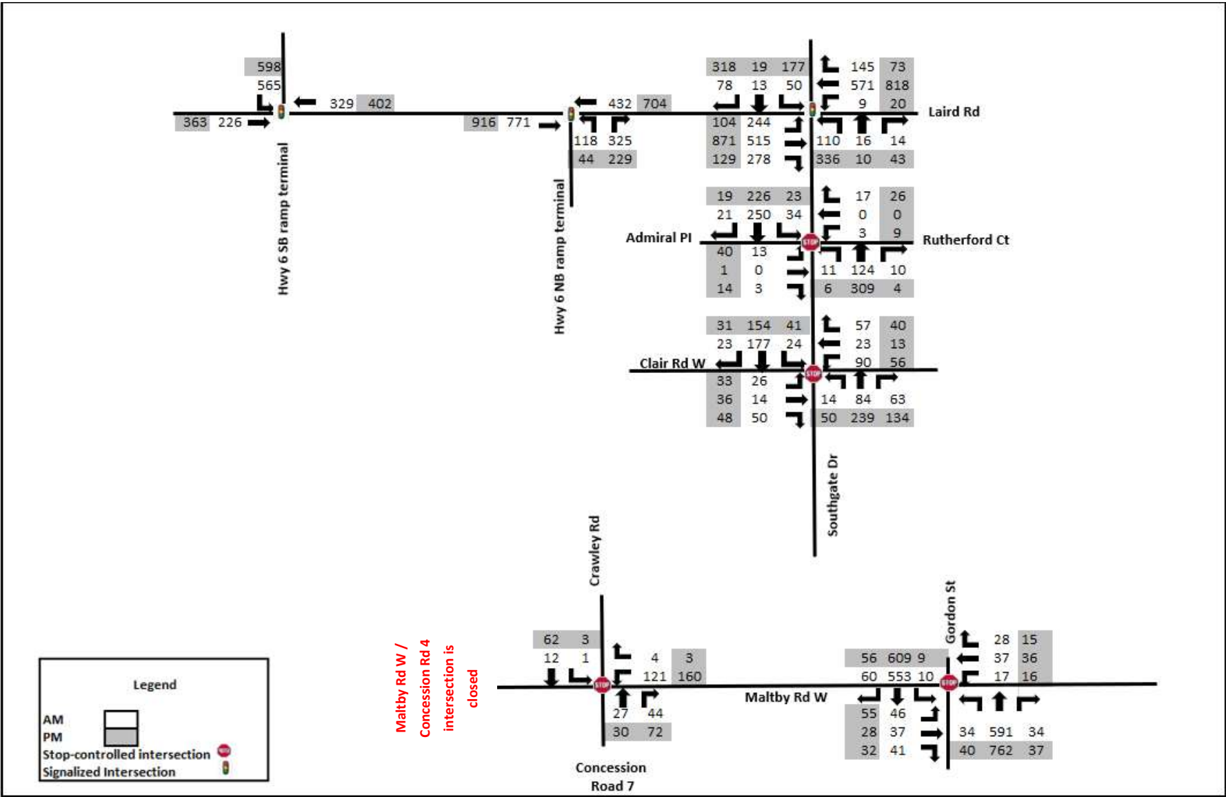
Figure 14: 2029 Background Traffic Volumes (without Southgate Drive Extension)
