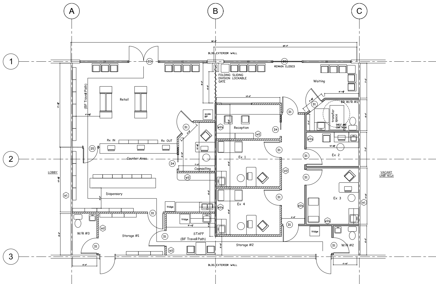
1 GROUND FLOOR PLAN A3 SCALE 1/4"=1'-0"
