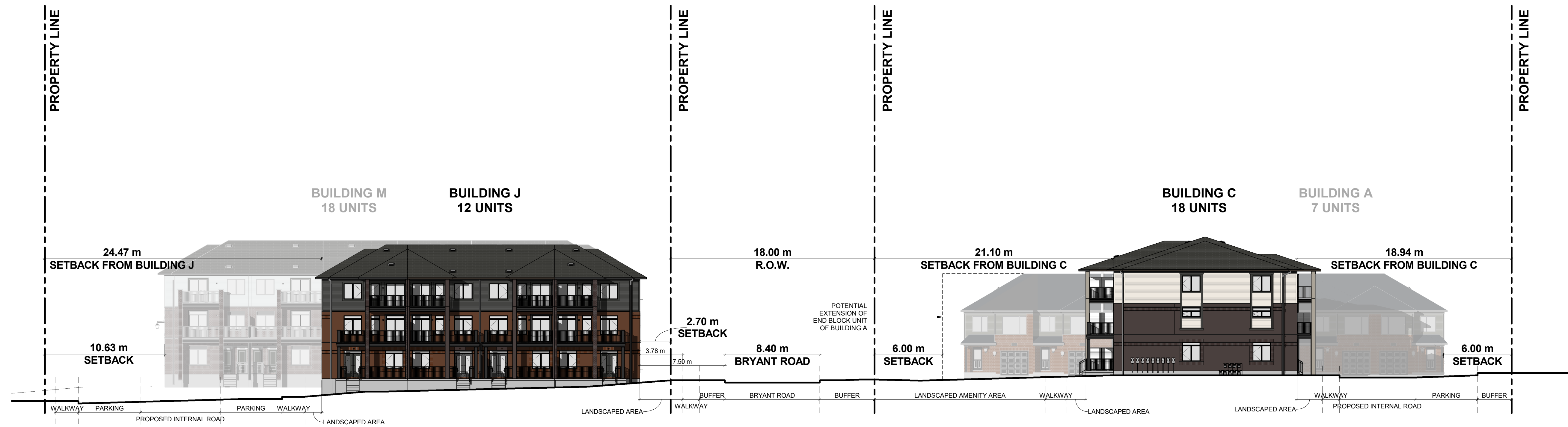
2 BRYANT ROAD SECTION 1:200
