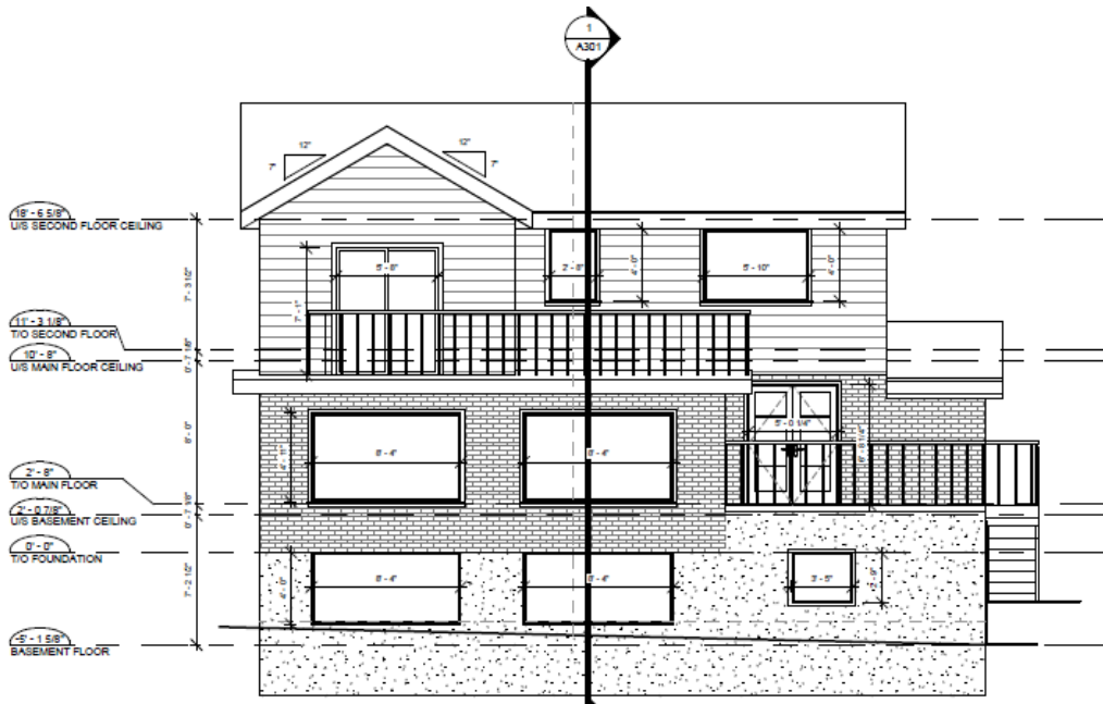
Figure 2: Proposed north elevation (rear)
