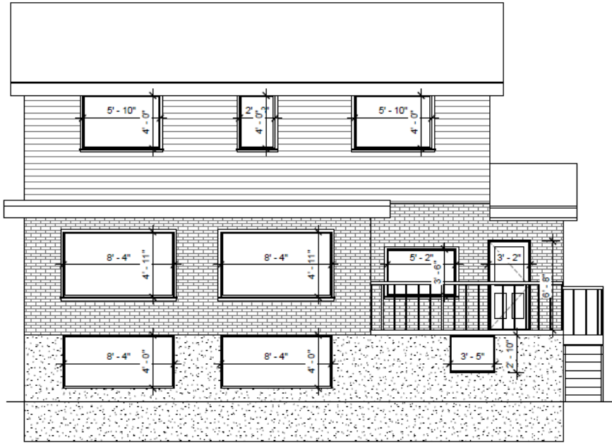
Figure 1: Existing North elevation (rear)
