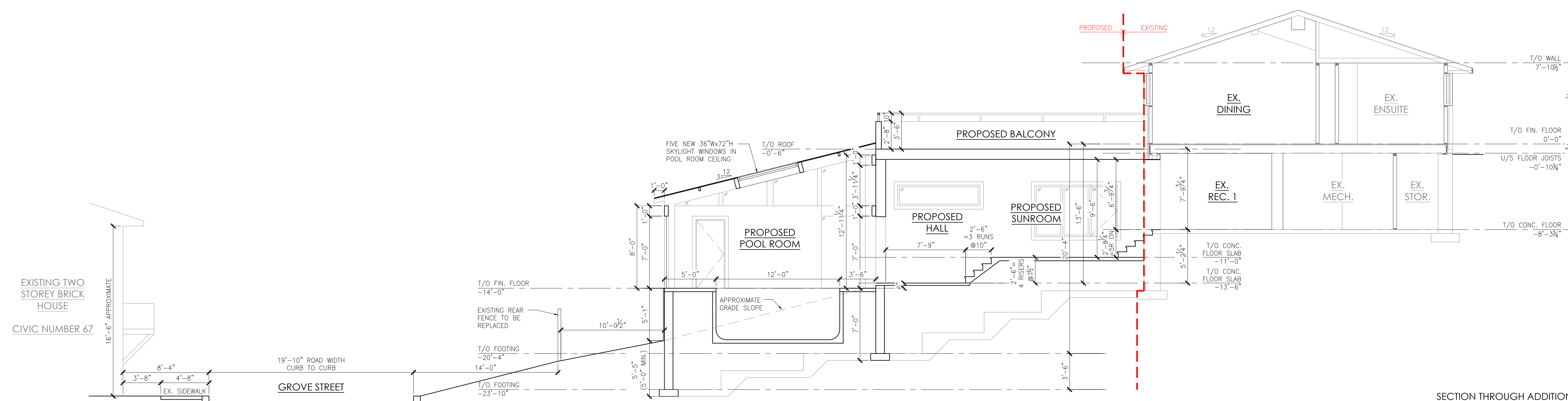
SECTION THROUGH ADDITION #3 1 3/16"=1'-0" A4.1
