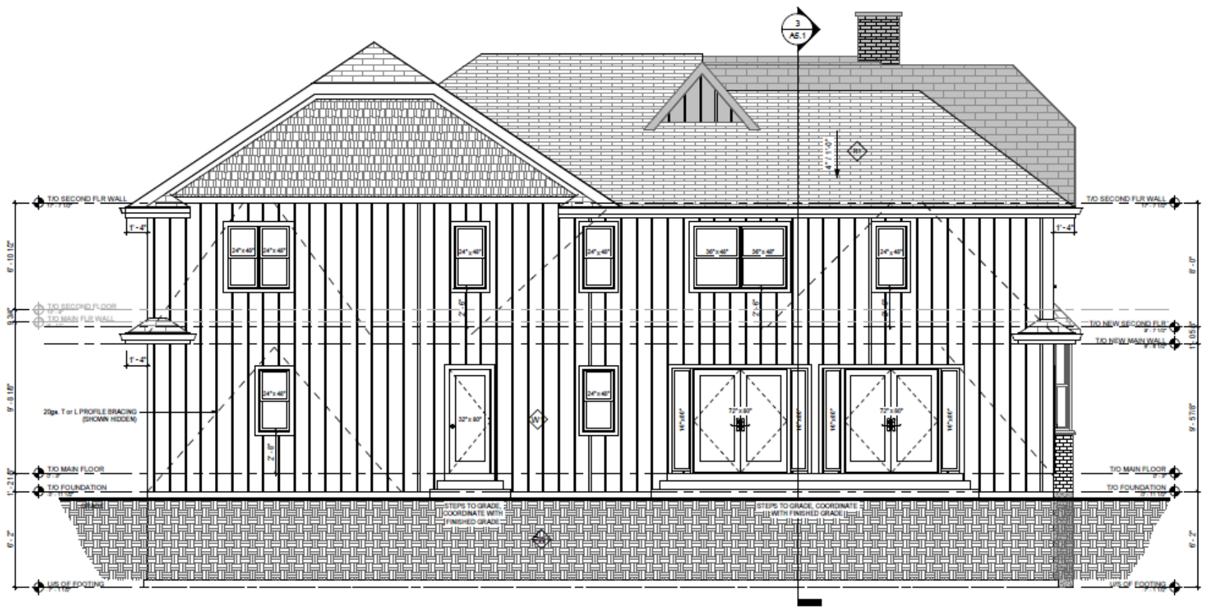
Figure 1: North Elevation showing proposed rear addition at 40 Spring Street
