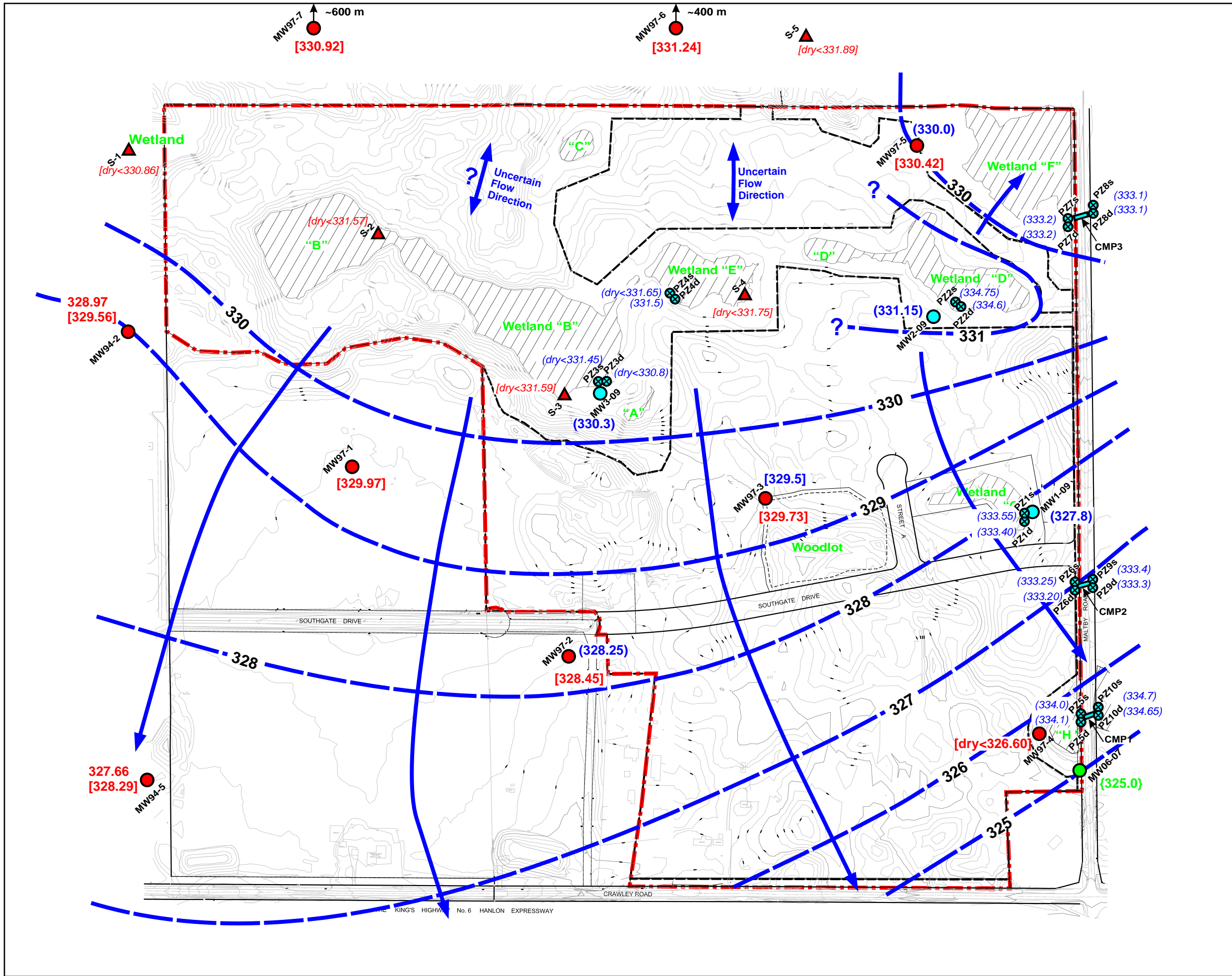
Figure 4 Interpreted 'Low' Water Table Configuration Hydrogeological Assessment for EIR, Southgate Business Park Guelph, Ontario Project No. 267
