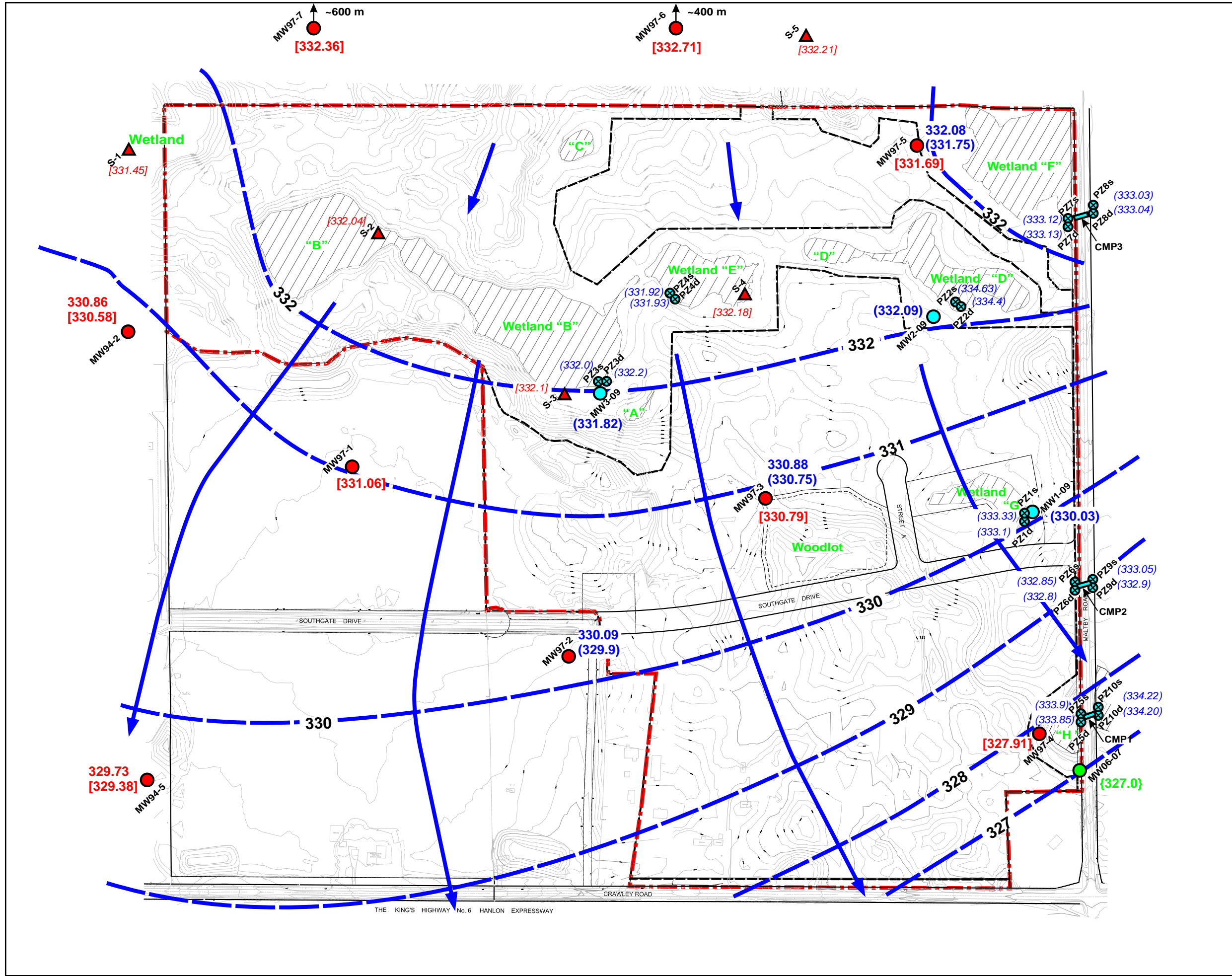
Figure 5 Interpreted 'High' Water Table Configuration
