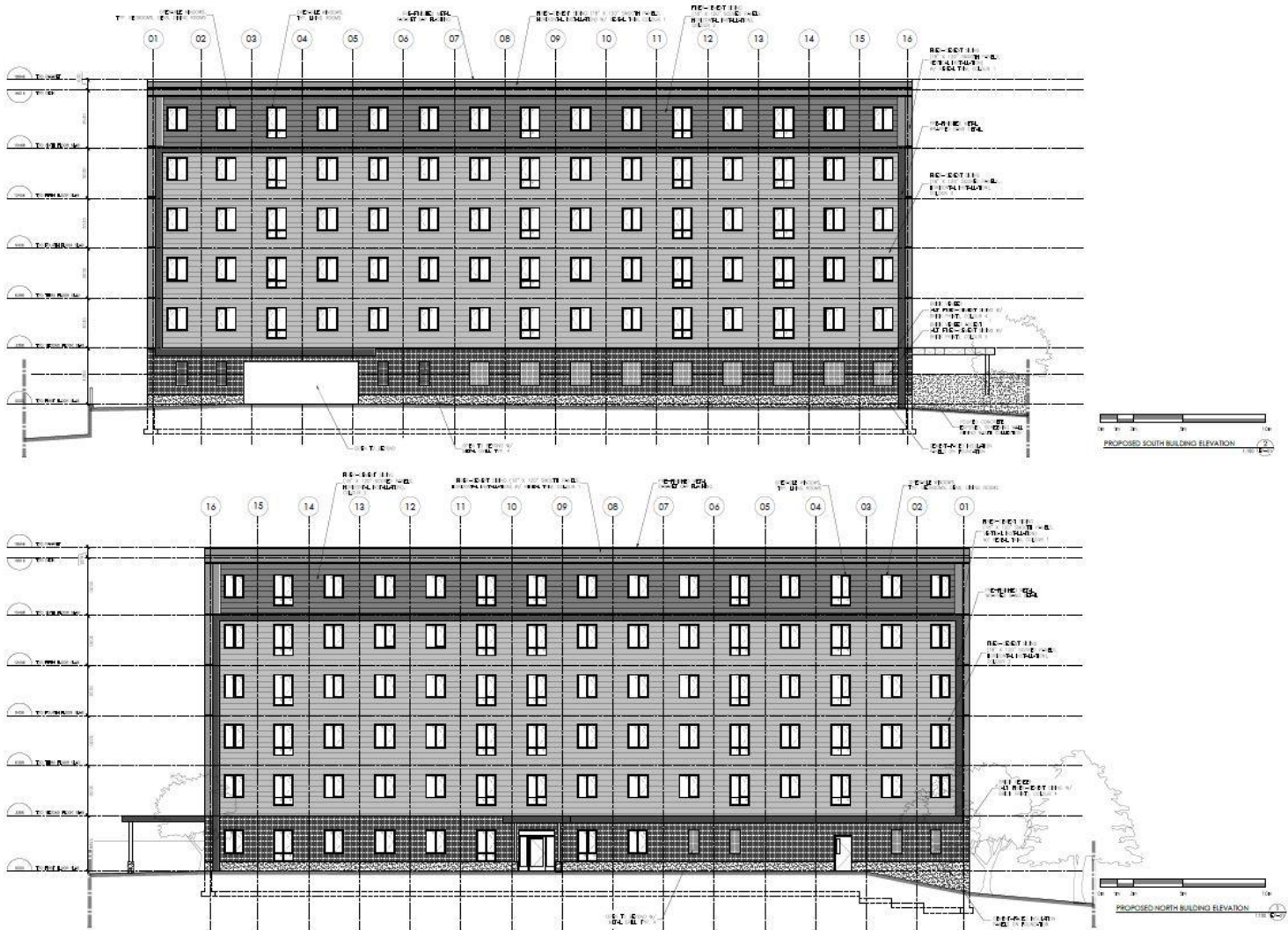
Figure 2: Apartment Building North and South Elevations – 303-317 Speedvale Avenue East
