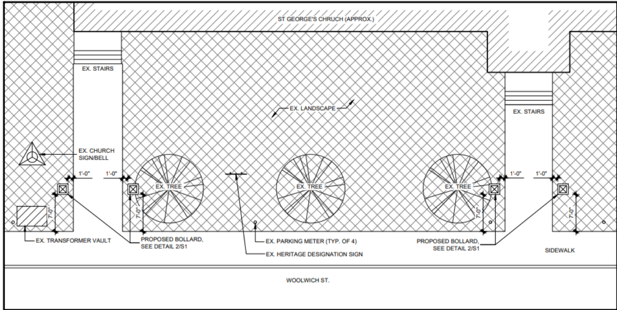
1 PARTIAL PLAN - SITE S1 SCALE: 3/32" = 1'-0"
