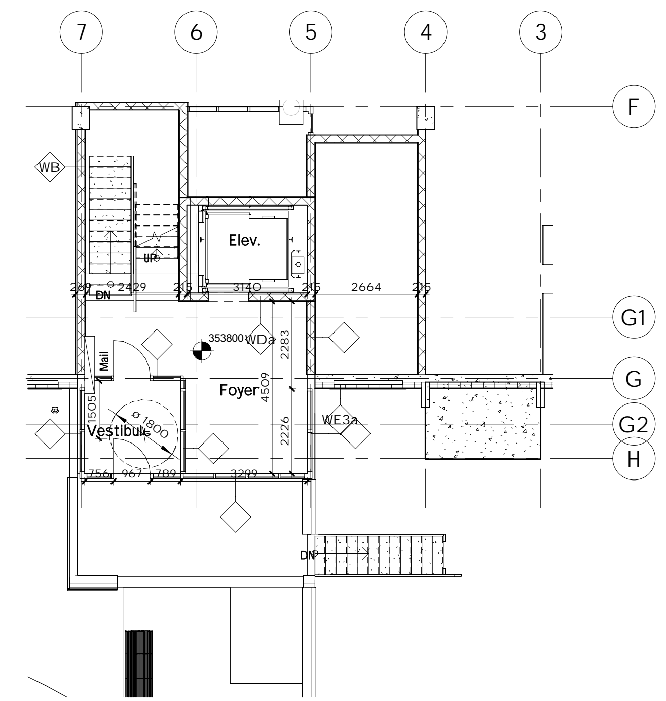
2 Main Entrance Floor Plan EP-2 1 : 100
