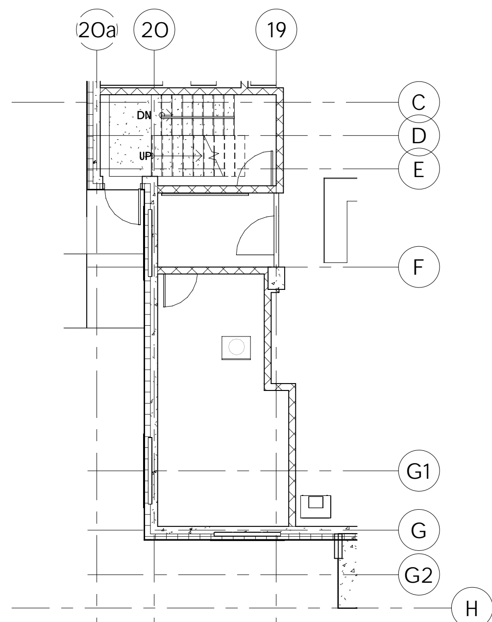
3 South Exit Floor Plan EP-2 1 : 100
