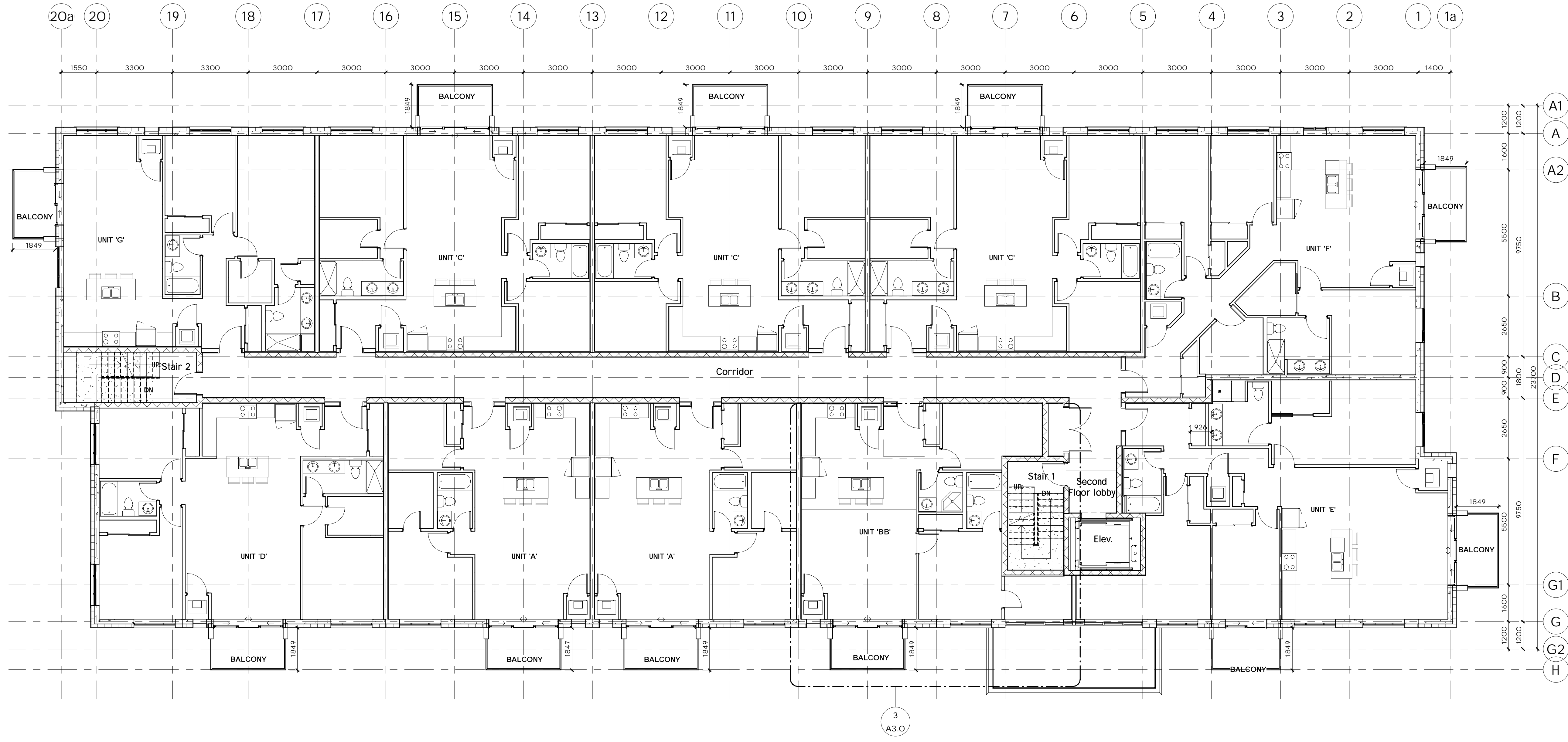
1 Second Floor Plan EP-3 1 : 100
