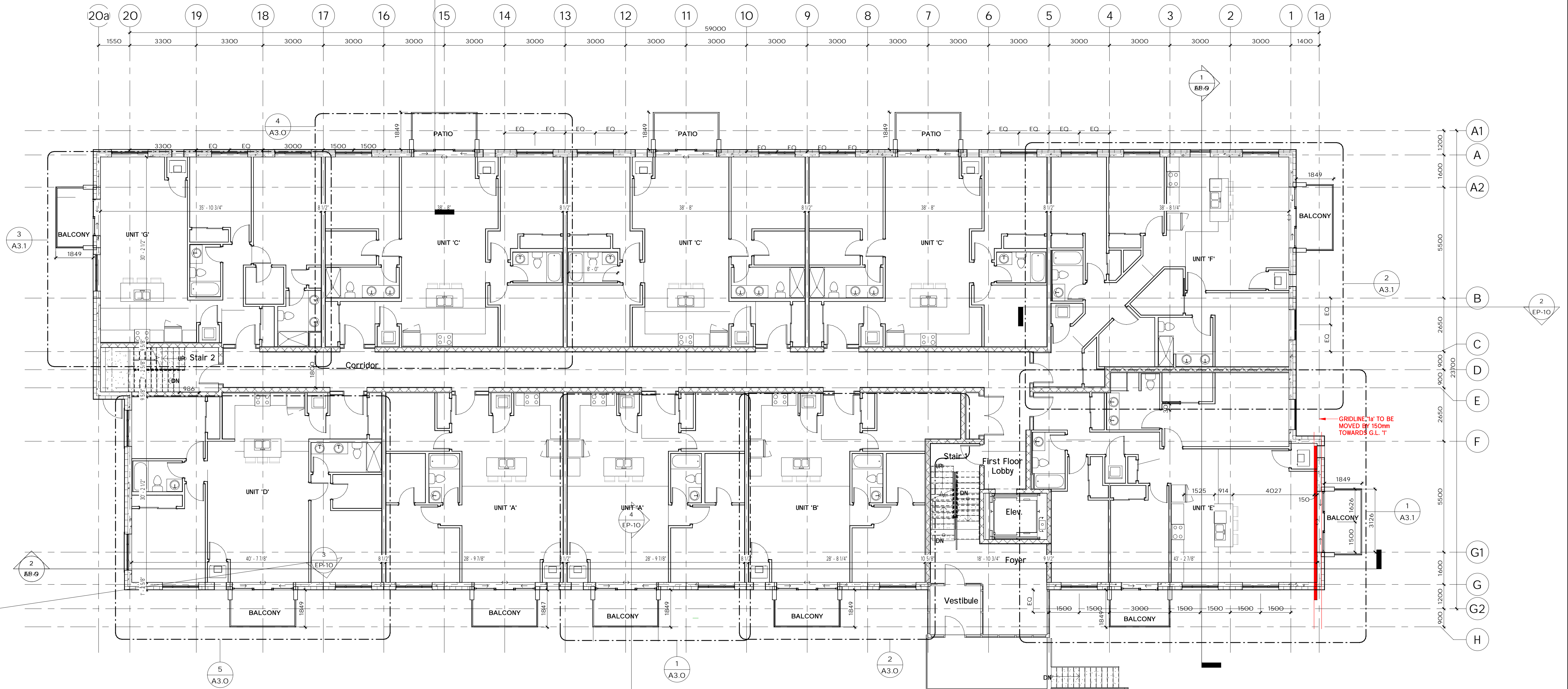
1 First Floor Plan EP-2 1 : 100
