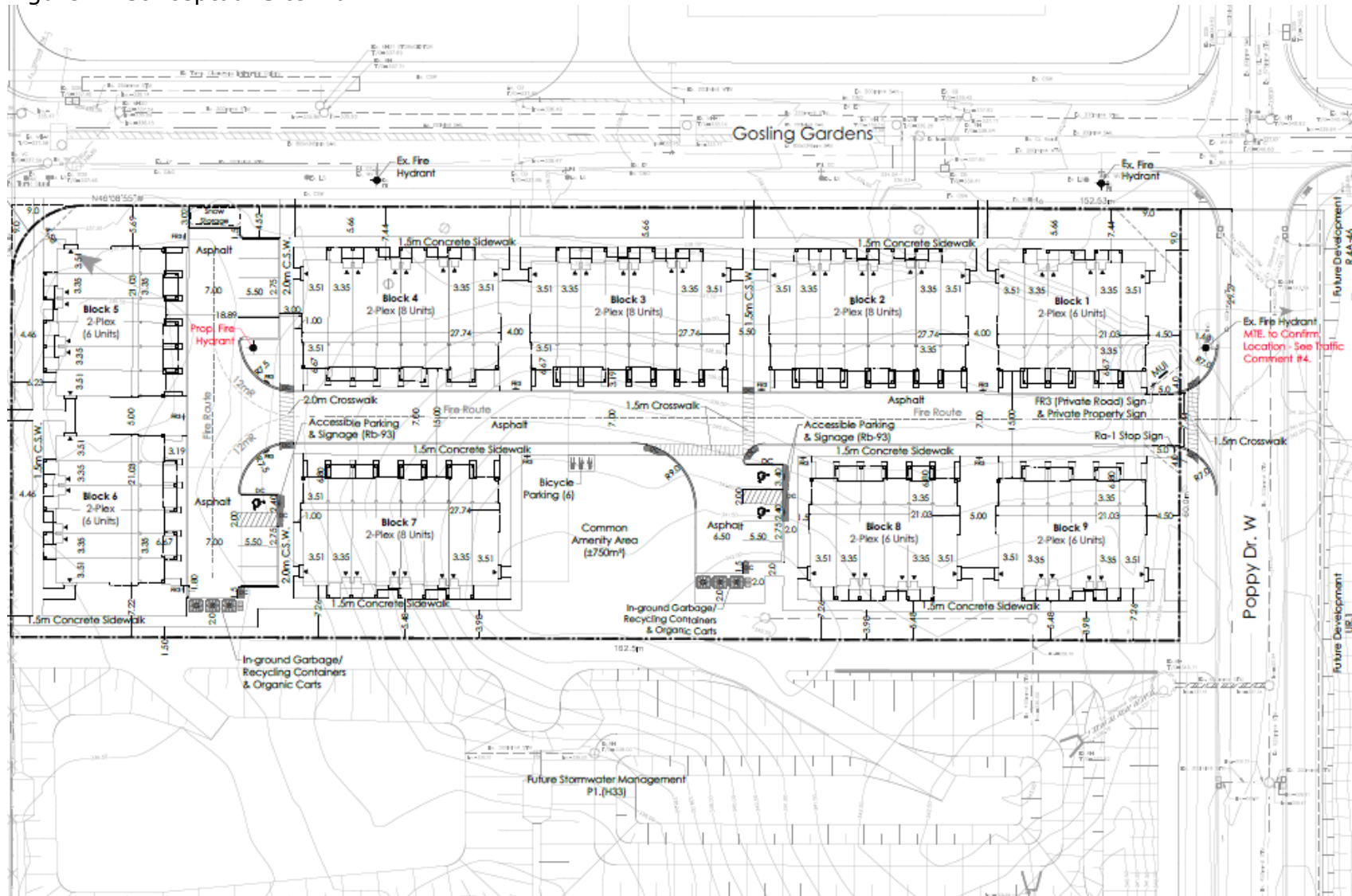
Figure 1: Conceptual Site Plan
