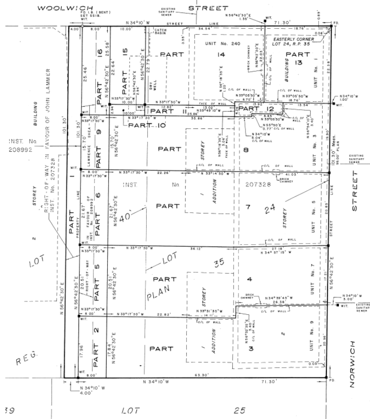
Figure 5 (City of Guelph) - Detail from Plan of Survey 61R-2027 showing 7 Norwich Street West as Parts 4 and 5. (Black, Shoemaker, Robinson & Donaldson Ltd., 1979)
