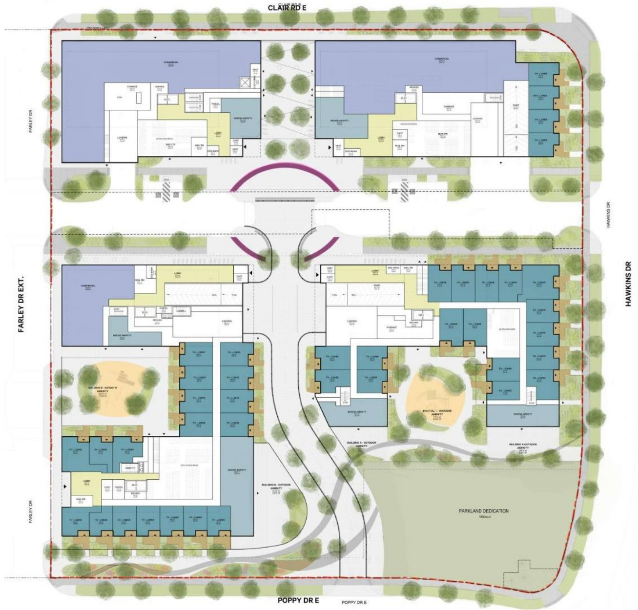
Figure 1: Conceptual Site Plan
