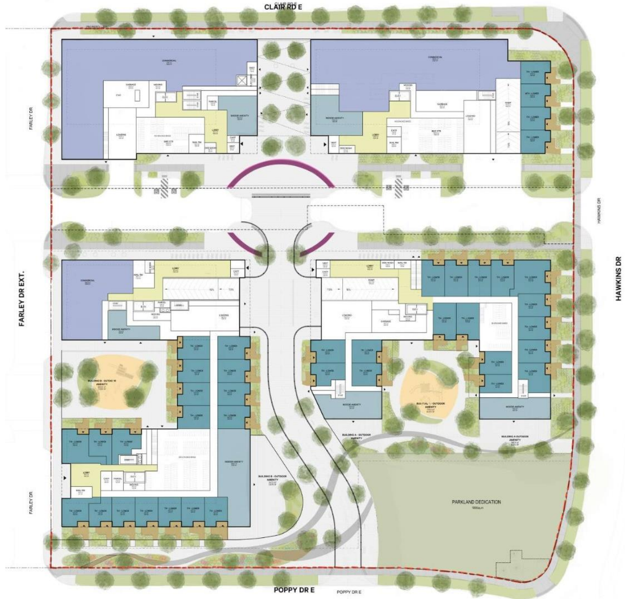
Figure 1: Conceptual Plan
