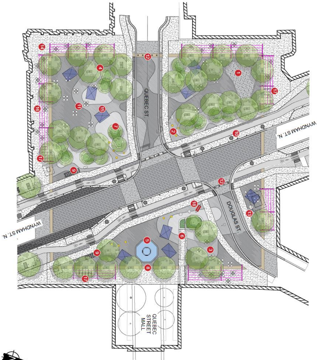
Figure 1: Plan view of the proposed design for St. George's Square
